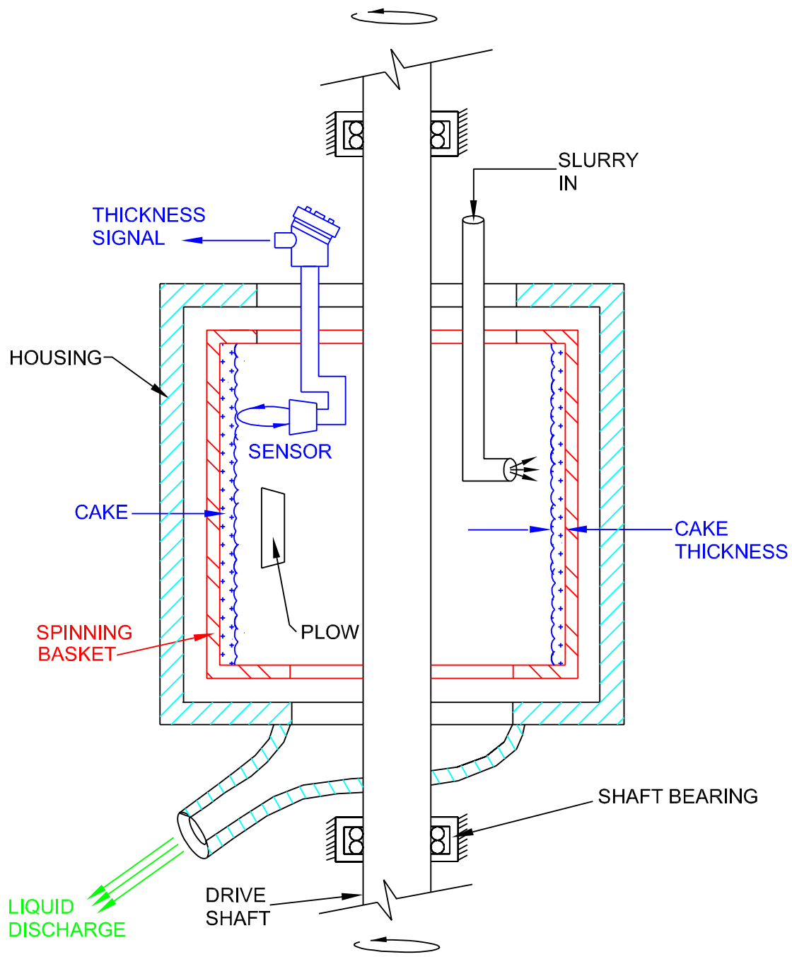
CONTINUOUS MEASUREMENT OF CAKE THICKNESS IN LARGE INDUSTRIAL CENTRIFUGES (SCHEMATIC) -M/N 858 ULTRASONIC SYSTEM IN SERVICE AT ALBERMALE (ORIGINALLY ETHYL CORP).
